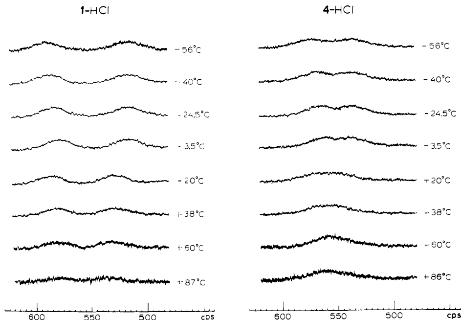
Figure 1. Temperature dependence of the resonance signal of the \text{NH}_2^+ protons of 1-(isopropylamino)-3-(3-methylphenoxy)-2-propanol hydrochloride (1·HCl) and 2-(isopropylamino)-3-(3-methylphenoxy)-1-propanol hydrochloride (4·HCl), measured in \text{CDCl}_3 .
