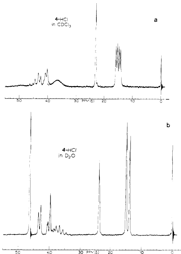
Figure 3. Part of the ^1\text{H} NMR spectra of 2-(isopropylamino)-3-(3-methylphenoxy)-1-propanol hydrochloride (4-HCl) measured in \text{CDCl}_3 (a) and \text{D}_2\text{O} (b).
