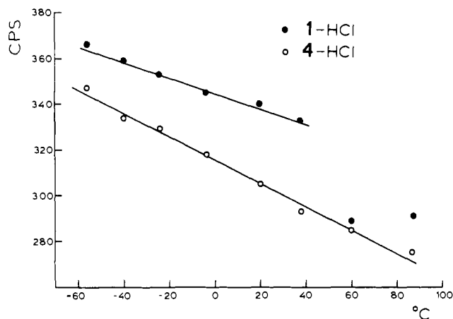
Figure 2. Temperature dependence of the resonance signal of the OH proton of 1-(isopropylamino)-3-(3-methylphenoxy)-2-propanol hydrochloride (1·HCl) and 2-(isopropylamino)-3-(3-methylphenoxy)-2-propanol hydrochloride (4·HCl), measured in \text{CDCl}_3 .
